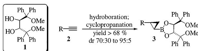
Scheme 1. Synthesis of stable, enantiomerically pure trans -cyclopropylboronic esters 3
