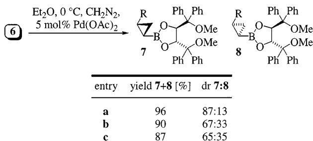
Scheme 3. Diastereoselective cyclopropanation of 6 to yield 7 and 8
