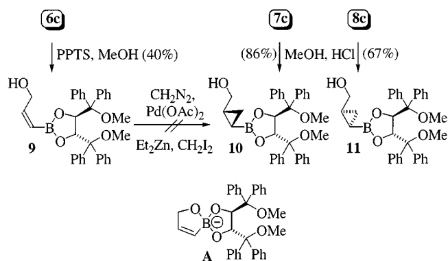
Scheme 4. Synthesis of hydroxymethylcyclopropylboronic esters 10 and 11
