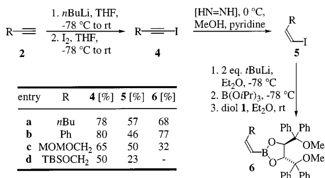
Scheme 2. Synthesis of cis -alkenylboronic esters 6 (MOM = methoxymethyl, TBS = t BuMe 2 Si)
