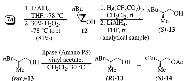
Scheme 5. Determination of the absolute configuration of cyclopropylboronic ester 7a by chemical correlation
